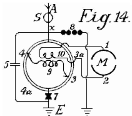
Fig.14 is a modified form of Fig.13 with inductive coupling.
