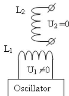
Fig.1 These orthogonal coils do not interact.
