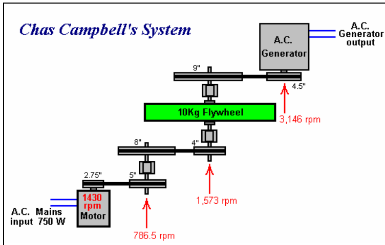
Figure 8.1 The Belt and Flywheel setup of the Chas Campbell Electricity Magnifier from the overunity forum.
