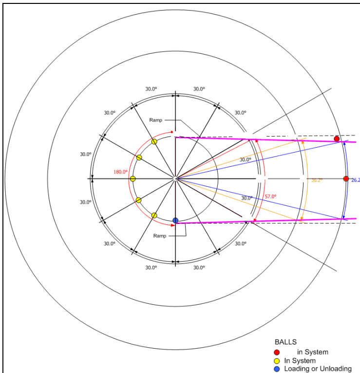
Figure 7.1 The conceptual picture of the Campbell wheel.
